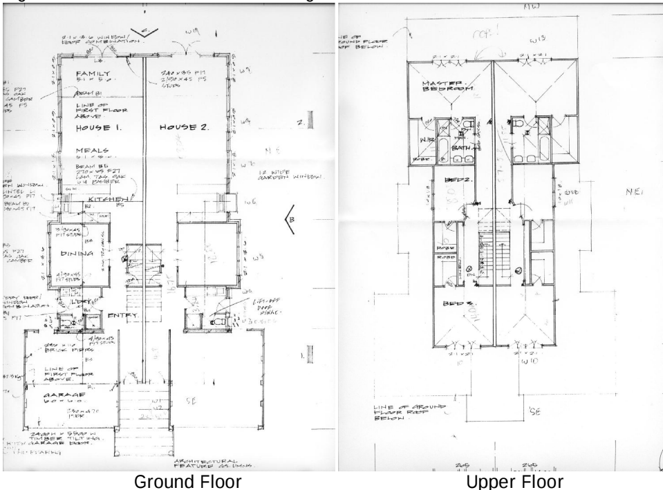
Figure 3.3: Semi Detached Dwelling
